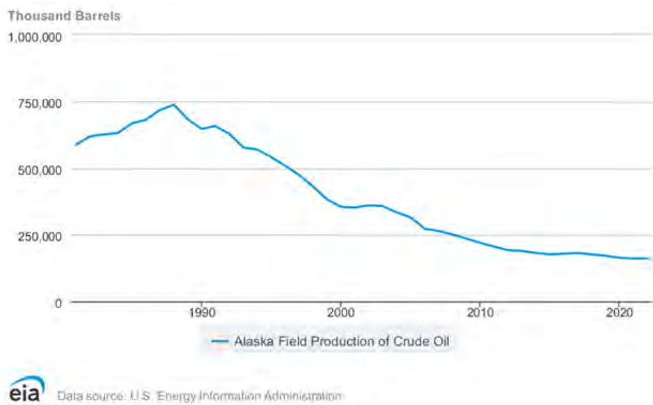
Figure 4. Alaska field production of crude oil (EIA, 2023).
