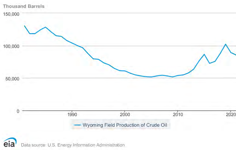
Figure 5. Wyoming field production of crude oil.
