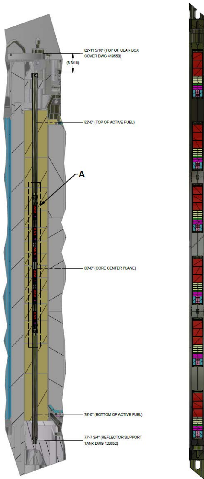
Figure 5.2. Elevation stack up of the TZM capsules in the ATR B2 position.
