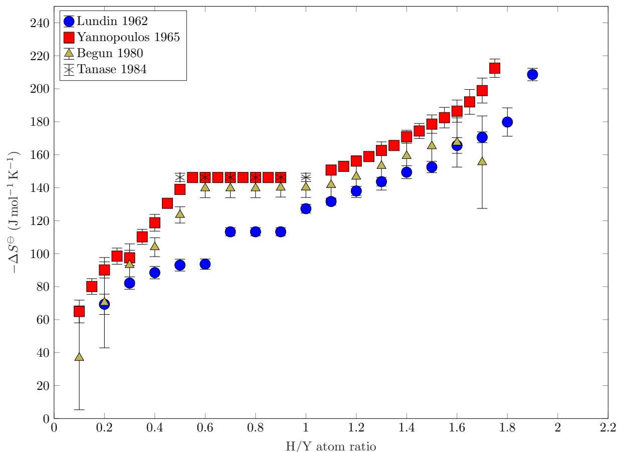
Figure 2.5: Partial molar non-configurational entropy of \text{YH}_x as a function of hydrogen content in H/Y units. Data taken from [9], [32], [37], [38].
