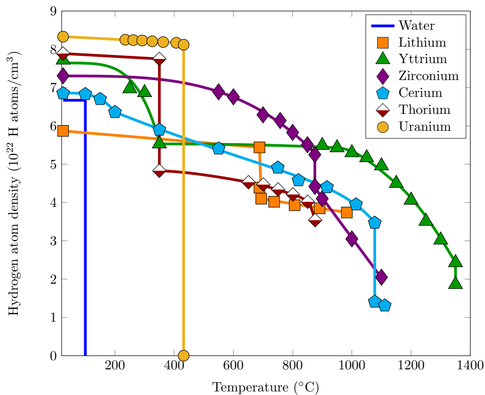
Figure 2.1: Hydrogen atom density as a function of temperature for water various metal hydrides in equilibrium with 1 atm of hydrogen gas for temperatures between 25 and 1400 °C (taken from [20]).
