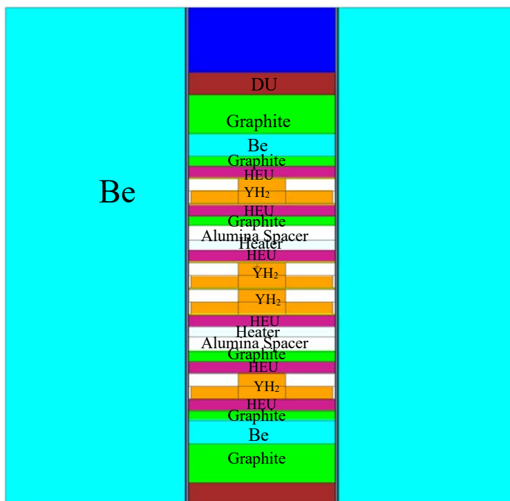
Figure 6.1. Critical experiment design overview.
