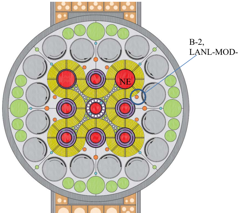
Figure 5.1: ATR core showing LANL-MOD-1 in the B2 position.
