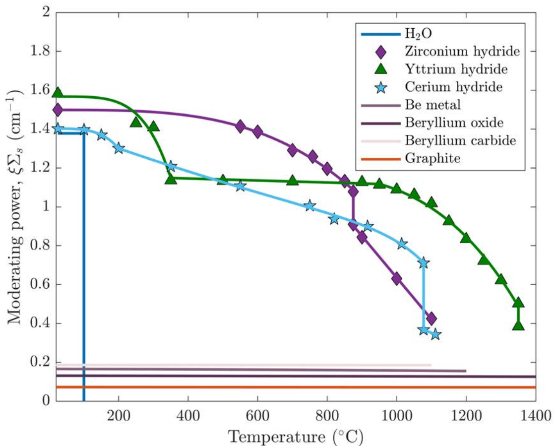
Figure 2.13: Moderating power as a function of temperature for various candidate moderator materials. All data points are taken from literature for materials at 1 atm pressure [9]–[11], [30], [32], [78]–[90]. Data for metal hydrides were determined for those materials under 1 atm of pure hydrogen.
