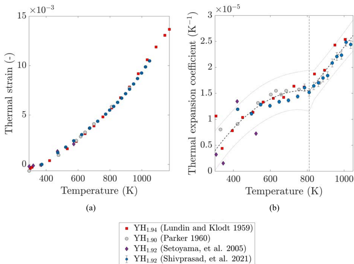
Figure 2.7: (a) Thermal strain and (b) thermal expansion coefficient for yttrium dihydride. Thermal expansion coefficient was fit to functions of temperature, the fitting parameters for which are summarized in Table 2.4. Figure adapted from [14].
