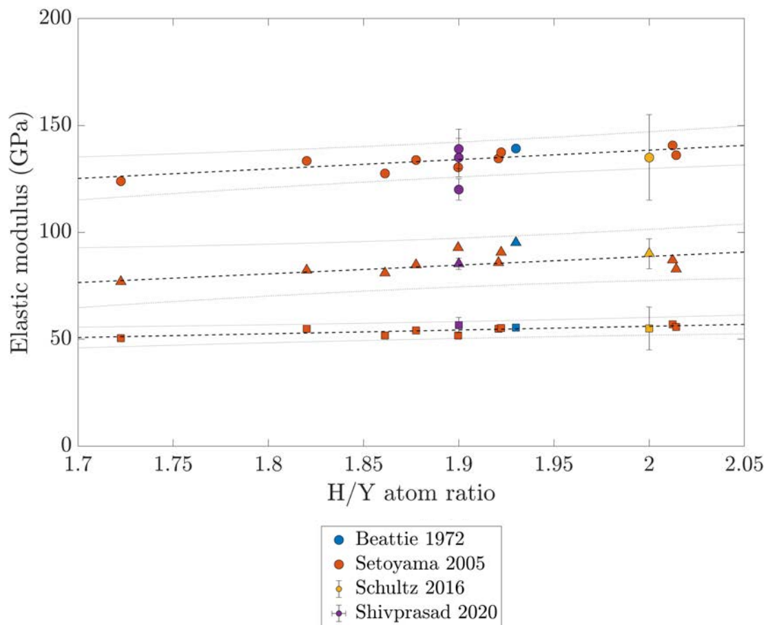
Figure 2.9: Shear, bulk, and Young's moduli as a function of hydrogen content for yttrium dihydride. Data from [11], [20], [23], [63]. Young's moduli are plotted in circles, bulk moduli are plotted in triangles, and shear moduli are plotted in squares.
