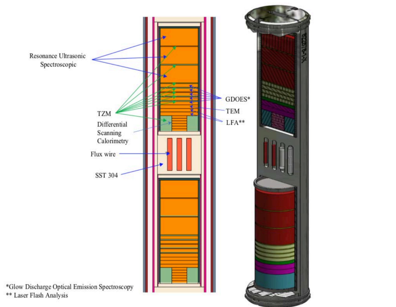
Figure 5.3. Hydride specimens located in a single ATR fixture basket. Two TZM inner capsules containing the hydride fit within a single ATR fixture, along with passive temperature and fluence monitors.
