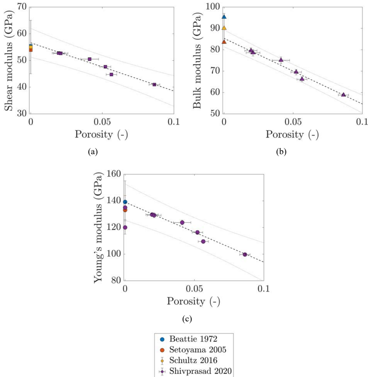
Figure 2.10: (a) Shear, (b) bulk, and (c) Young's moduli of yttrium dihydride as a function of porosity. Data from [11], [20], [23], [63].
