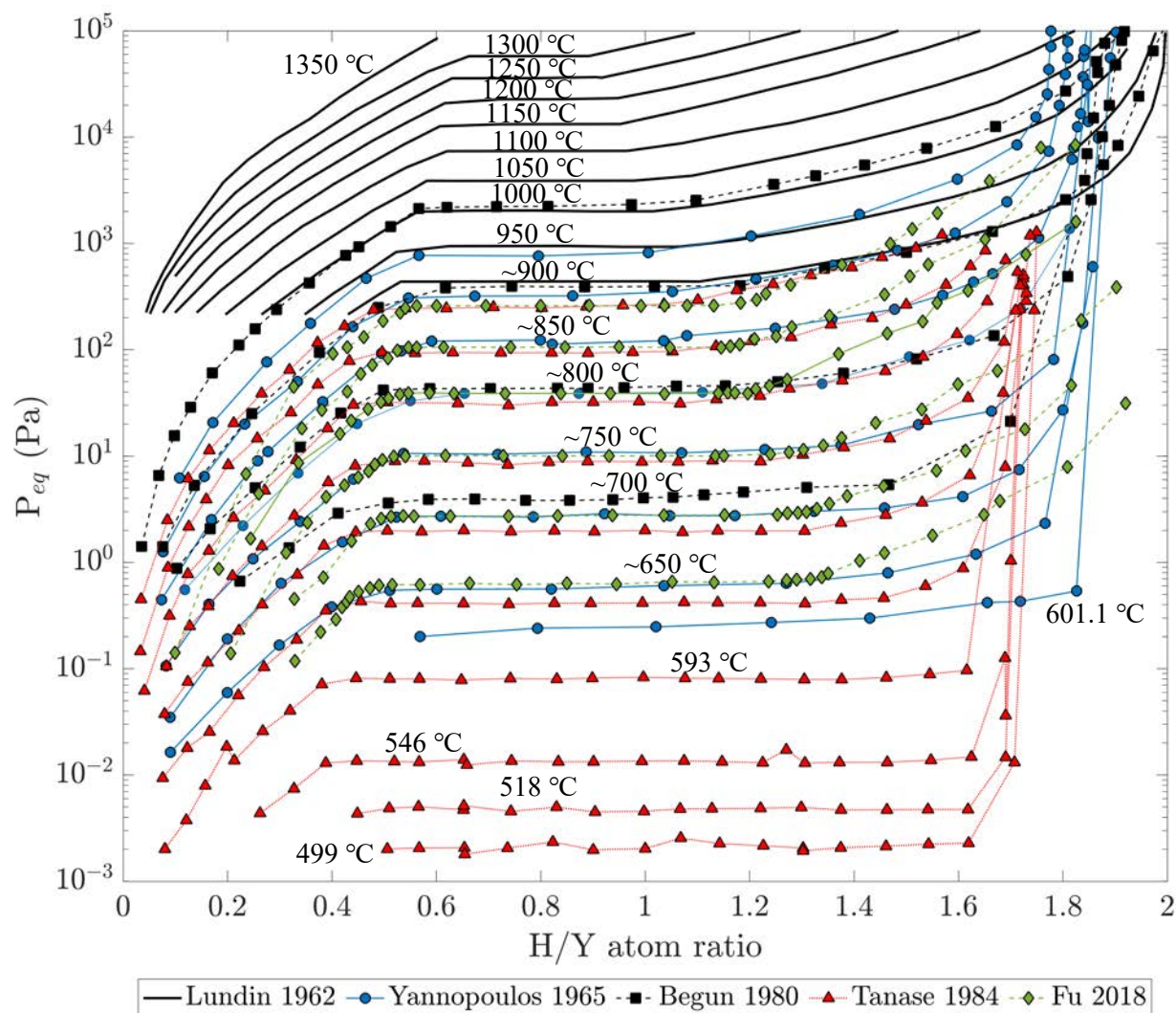
Figure 2.2: Compilation of PCT curves for the Y-H system up to a hydrogen-to-yttrium ratio of 2.0. Data replotted from [9], [32], [33], [37], [38].
