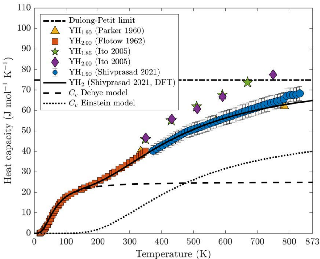
Figure 2.6: Molar heat capacity of yttrium dihydride as a function of temperature. Data from [13]–[16].
