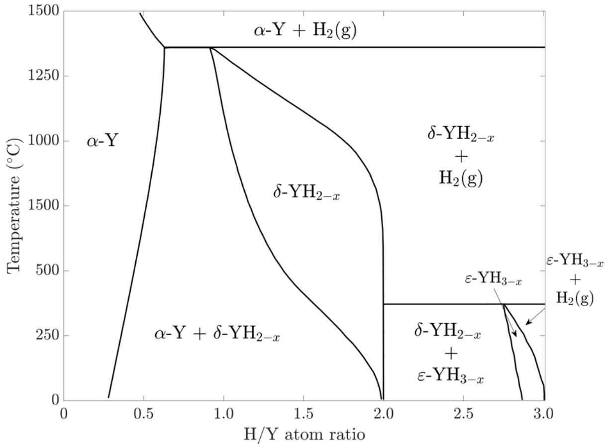
Figure 2.3: Redrawing of the Y-H phase diagram based on CALPHAD analysis by Peng, et al. [40]. Phase regions are labeled and phase regions have been modified from the original source as a function of H/Y atom ratio.
