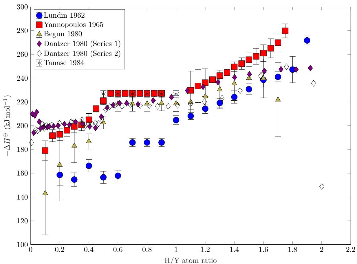
Figure 2.4: Partial molar enthalpy of formation for YH_x as a function of hydrogen content in H/Y units. Data taken from [9], [32], [37], [38], [47].
