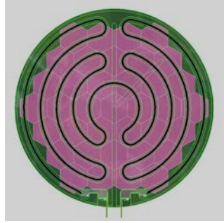
Figure 6.3. Alumina and graphite heater to be used in integral critical experiments at NCERC.
