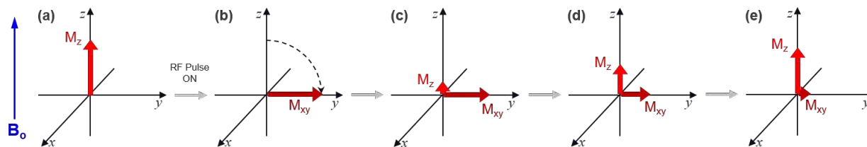
Figure 2.11: Magnetization evolution before and after a pulse of RF radiation is applied. The applied magnetic field is in the direction of the z-axis.
