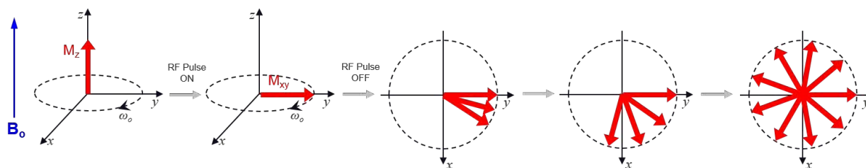
Figure 2.12: Loss of coherence of magnetization in the x-y plane after an RF pulse is applied.
