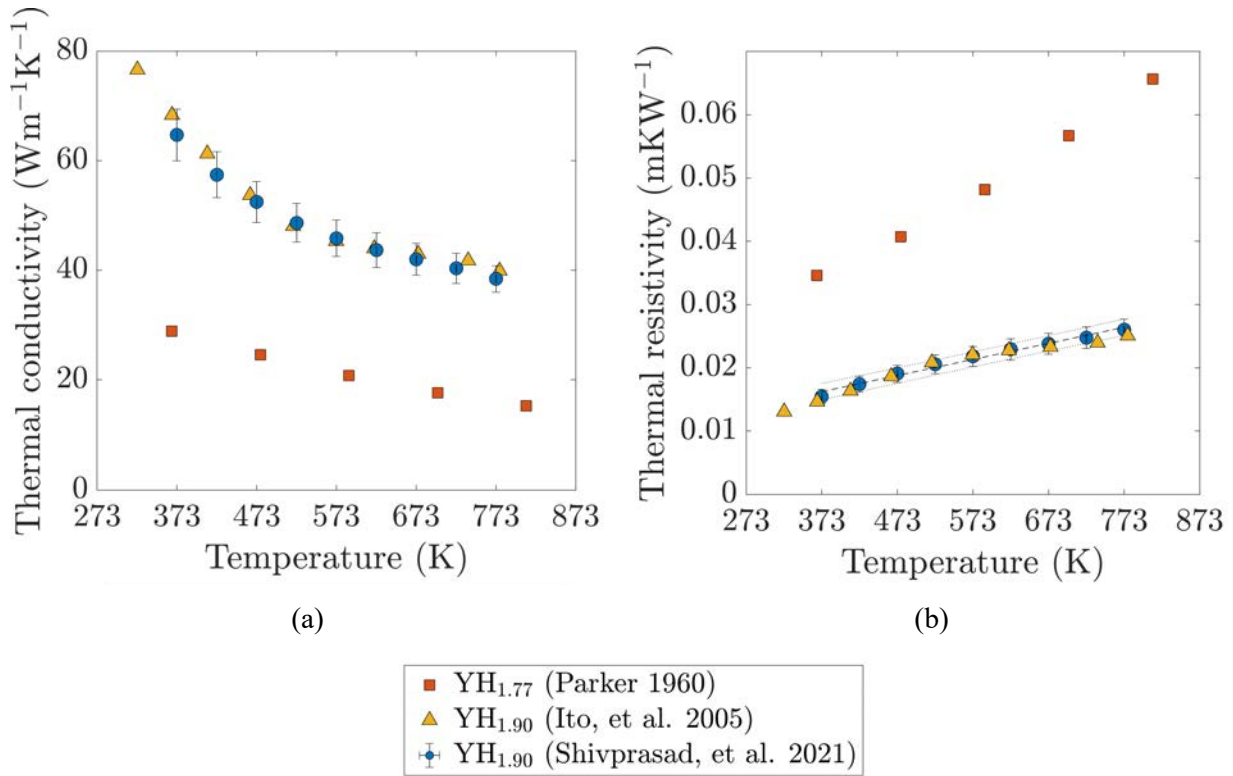
Figure 2.8: (a) Thermal conductivity and (b) thermal resistivity for yttrium dihydride as a function of temperature. Data from [13], [14], [16].
