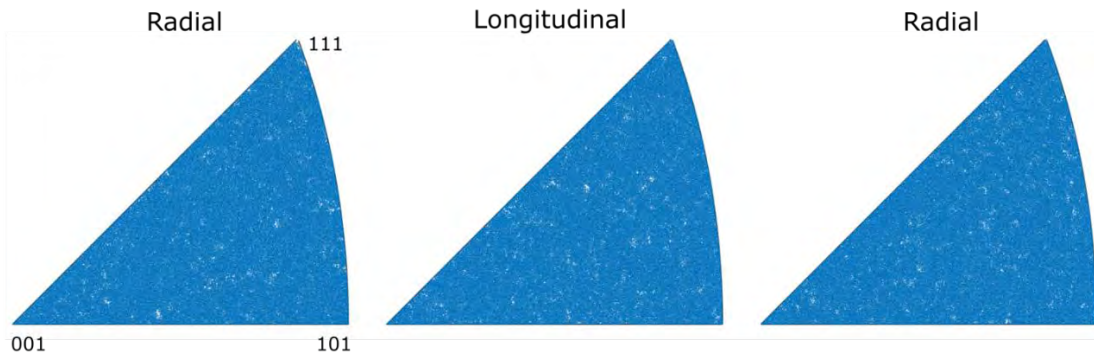
Figure 3. IPFs of EBSD data from the as-received PM HIP bar.
