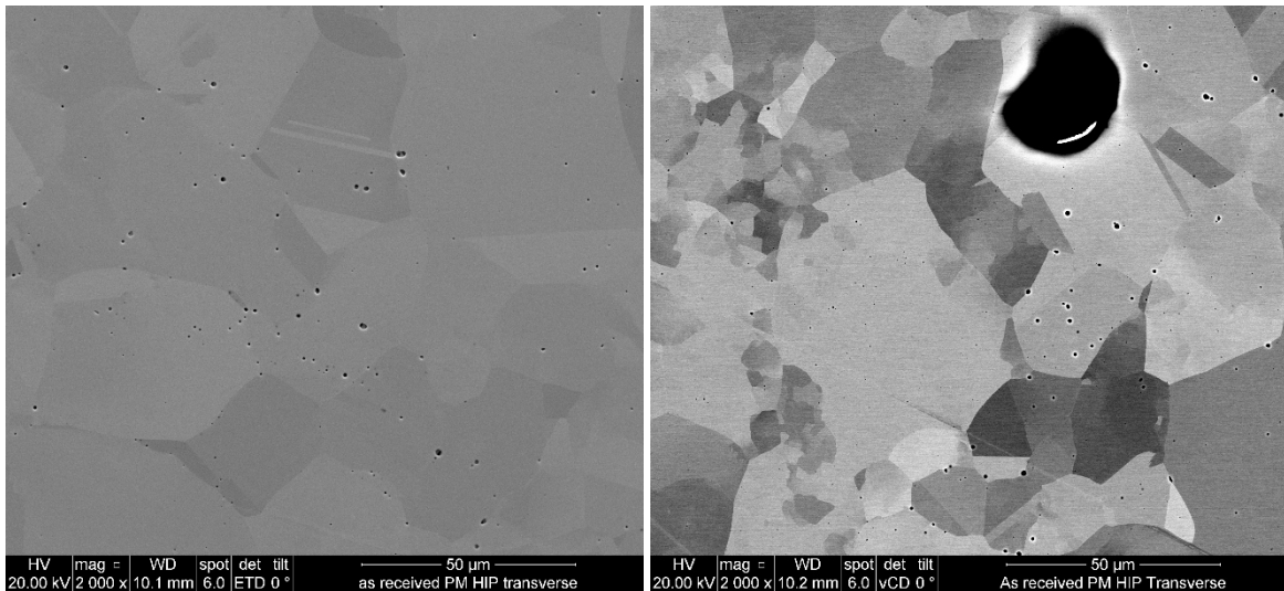
Figure 1. SE image (left) and BSE image (right) of the as-received PM HIP at a magnification of 2,000×. Porosity is present in the as-received PM HIP. There is a wide distribution in porosity size.
