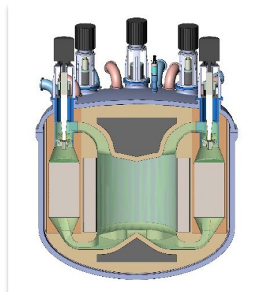
Molten Chloride Fast Reactor
