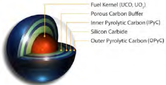
A tri-structural isotropic or “TRISO” fuel particle
