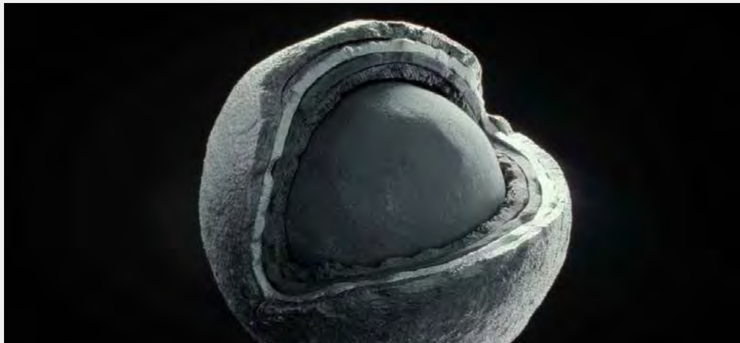
TRISO: A fuel “pebble” of the type most commonly planned for high temperature gas reactors but can also be used in other reactor designs (see some micro-reactor designs and FHR designs). These pebbles, which range in size from ping pong balls to tennis balls, contain particles of uranium or other fissile fuels, coated in silicon carbide or other heat-tolerant materials (see figure above). Photo Source: USNC
