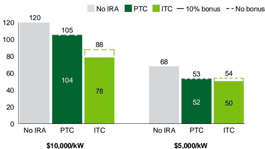
Figure 25: The ITC has greater impact for projects with higher construction cost versus the PTC 100,101
