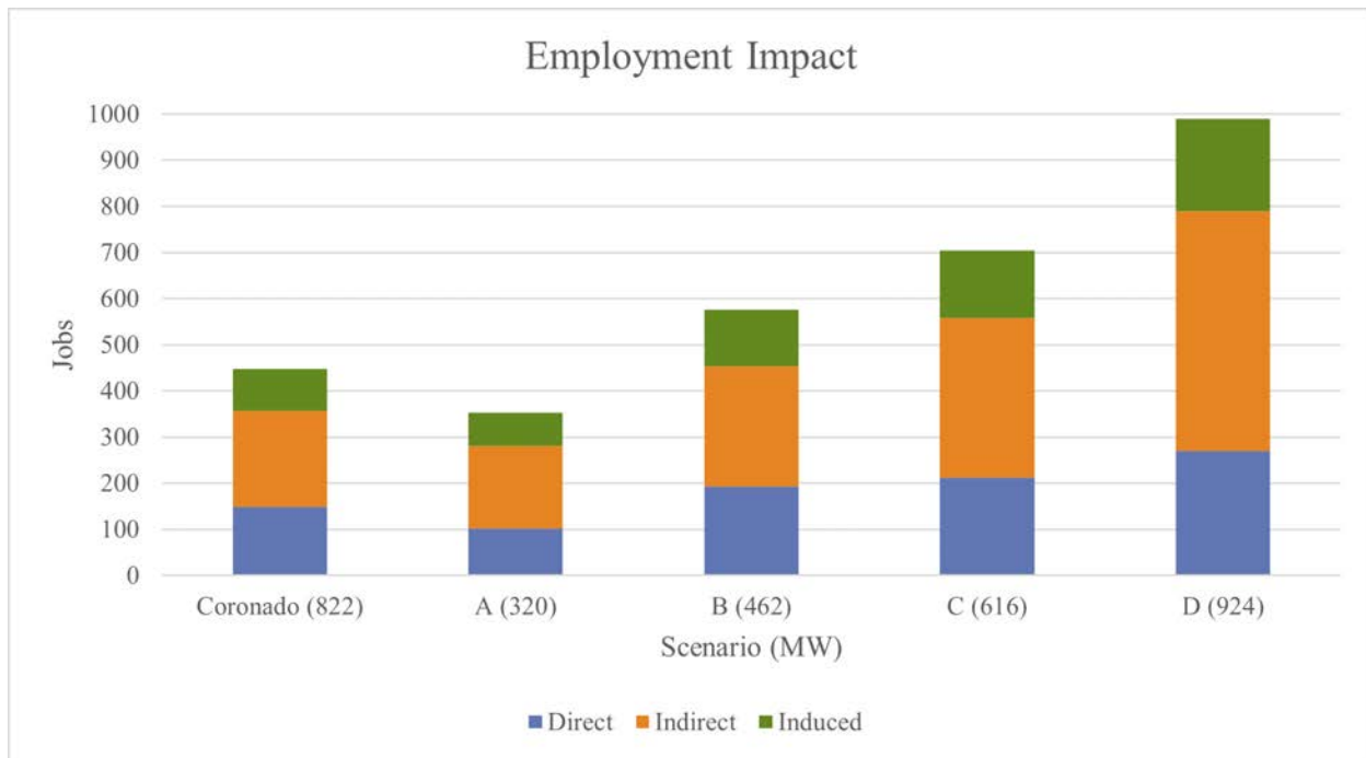
Figure 9. Employment Impact.
