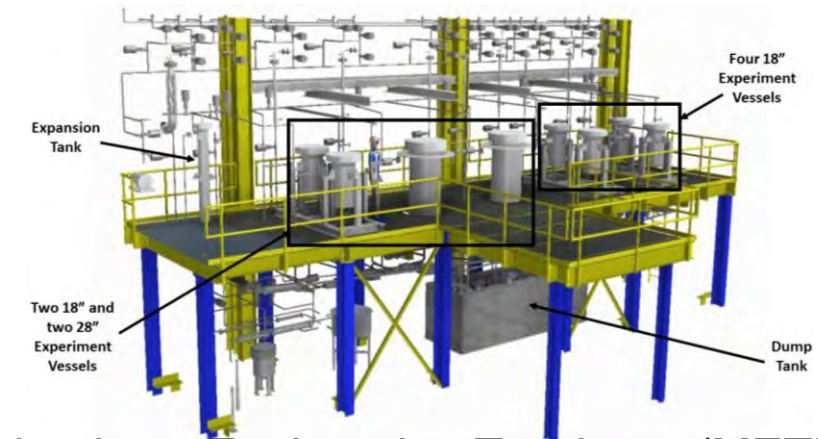
Mechanisms Engineering Test Loop (METL)
